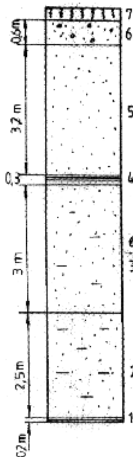
Fig. 1 Geological log of the outcrop with the fauna from the Erghevita Valley
